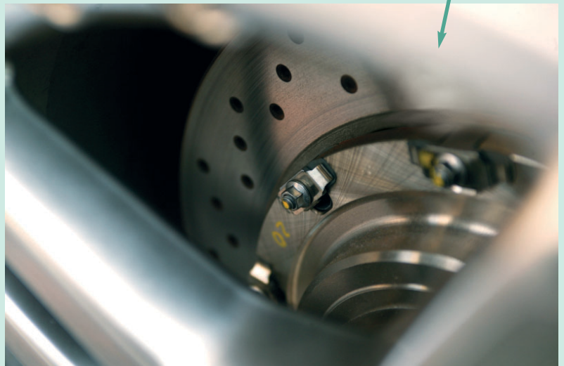
AMG compound braking system with two-piece rotor and hub assembly
